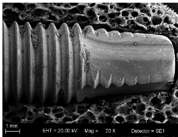
FIGURE 4. Scanning electron microscopy of the implant's apical region and surrounding bone (20x magnification): 400°C heat sample
