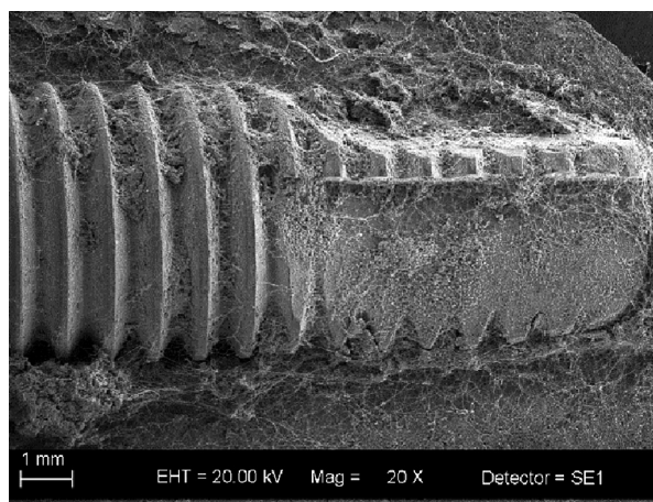
FIGURE 5. Scanning electron microscopy of the implant's apical region and surrounding bone (20x magnification): 30 days immersion sample
